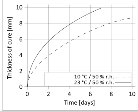
Diagram 1: Curing speed Sikaflex®-211 CN
