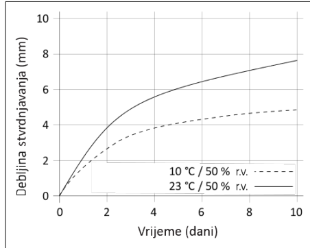
Diagram 1: Curing speed Sikaflex®-521 UV
