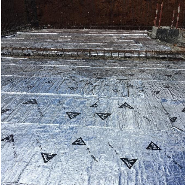
Picture: SikaBit® W-15 was applied on the floor retaining wall
