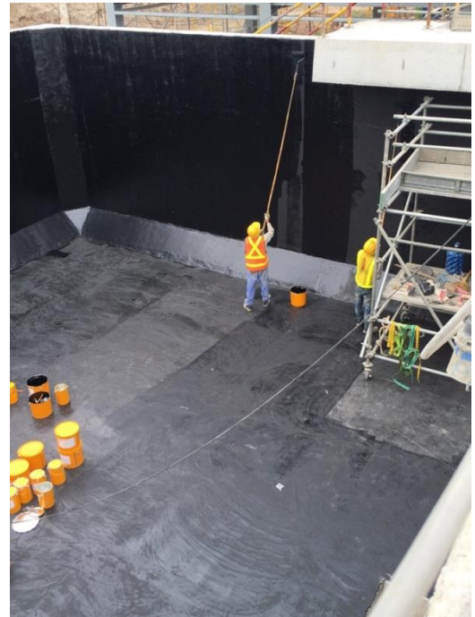
Picture: Sikafloor®-81 EpoCem® New HC was applied at Nestle Bong Sen with system of Sikafloor®-81 EpoCem, Sika® Poxita F
